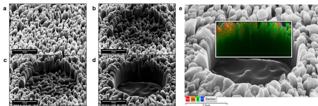
Fig. 5. (a) FIB-SEM images of the pellet area selected for the beam cross-section; images of the pruned rods by gallium ion beam with prune depth of (b) 0.5 \mu\text{m} , (c) 1.0 \mu\text{m} and (d) 3.0 \mu\text{m} , respectively, and (e) the area analyzed from the sum of all X-ray collected data during EDS acquisition. (A colour version of this figure can be viewed online.)
