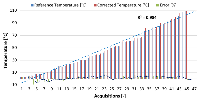
Fig. 5. Temperature curve with adjustment.
