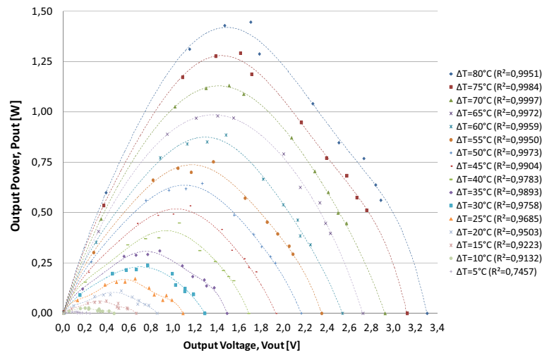
Fig. 16. The output power, P_{out} [W] versus the output voltage, V_{out} [V], for different temperature gradient, \Delta T [°C].
