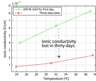
Fig. 7. Ionic conductivity measurement of the LiPON film as deposited and after 30 days of exposure to the atmosphere.
