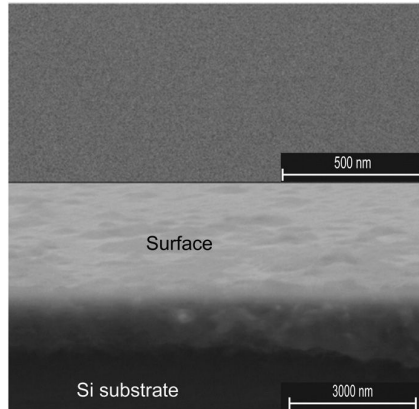
Fig. 6. A surface (top) and cross sectional (bottom) SEM image of a LiPON sample deposited under the best settings (150 W and 0.03 Pa). No crystalline structure was found in the surface.
