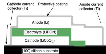
Fig. 1. An artwork of film battery with a solid-state electrolyte made of lithium-phosphorous oxynitride (LiPON). It must be noted that the thickness of each layer is not on scale for better visualization.
