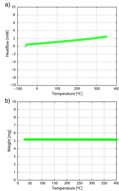
Fig. 8. a) Heatflow (mW) of the LiPON film as a function of temperature during DSC analysis. b) Weight of the LiPON film as a function of temperature during TGA analysis.
