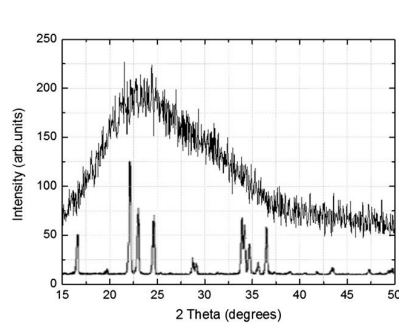
Fig. 5. X-ray diffraction patterns of the LiPON film (top line) and the Li_3PO_4 sputtering target (bottom line).
