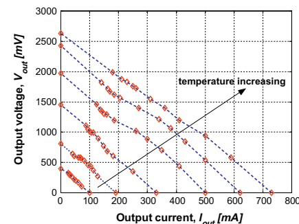
Fig. 3. The output voltage, V_{out} [mV], versus the output current, I_{out} [mA], for several test temperatures, T_{test} [°C].
