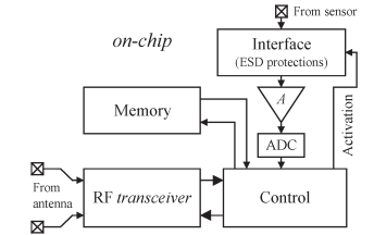
Fig. 8. Block diagram of microsystems for use in cars.
