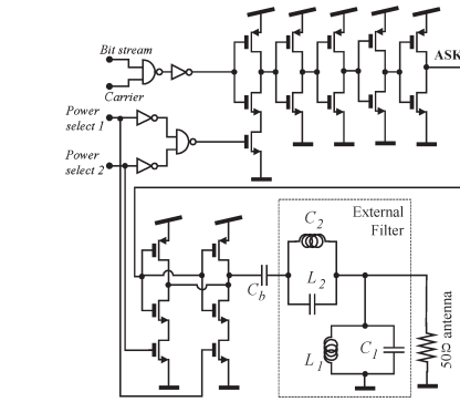
Fig. 4. Schematic of the transmitter.
