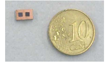
Fig. 9. Module photograph showing the electronics (microchip on the left), the RF transceiver (microchip on the right), and a planar antenna.
