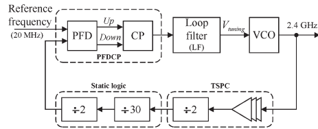
Fig. 5. PLL structure.
