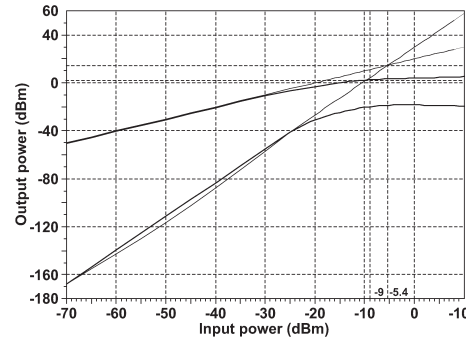
Fig. 6. IP1 and IP3 of the LNA.
