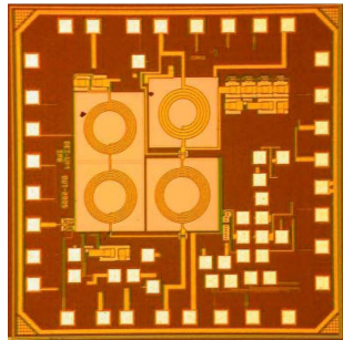
Fig. 10. Die photograph of the RF CMOS transceiver.
