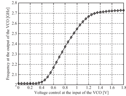
Fig. 7. Measured working characteristic of the VCO.
