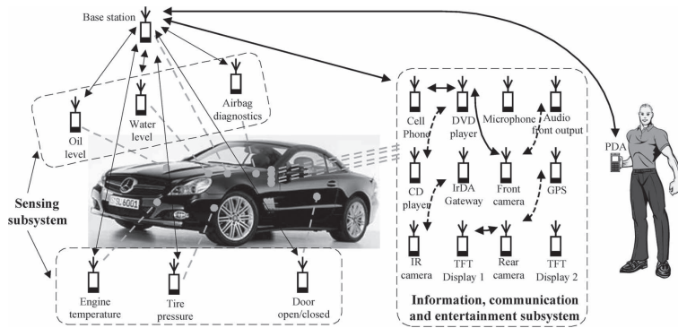
Fig. 1. System architecture using the CMOS-SRWSN.
