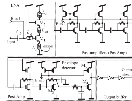
Fig. 3. Full schematic of the receiver.
