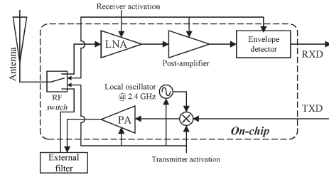
Fig. 2. Block schematic of the transceiver.
